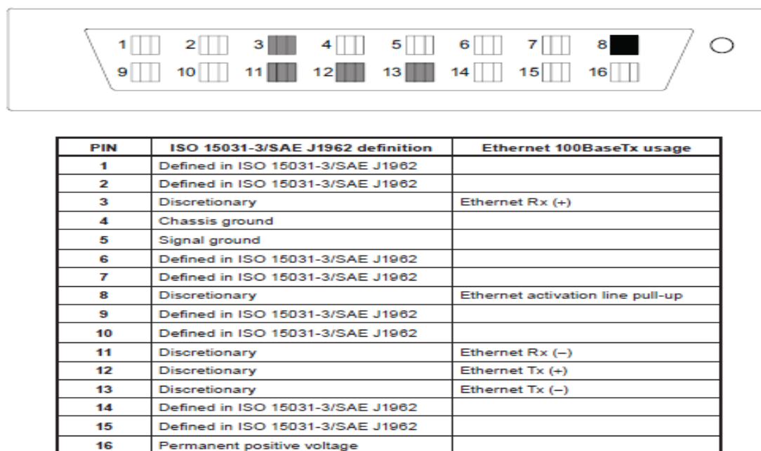
Figure 6: Example of pin-out for Ethernet recommended for 100BaseTx on the ISO15031-3/SAE J1962 diagnostic connector; taken from ISO 13400-3 17
